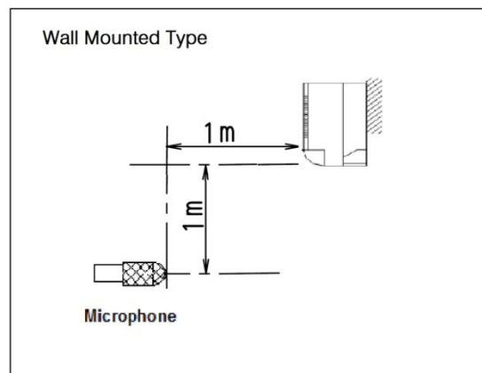
Figure 8.2: Wall mounted sound pressure level measurement
