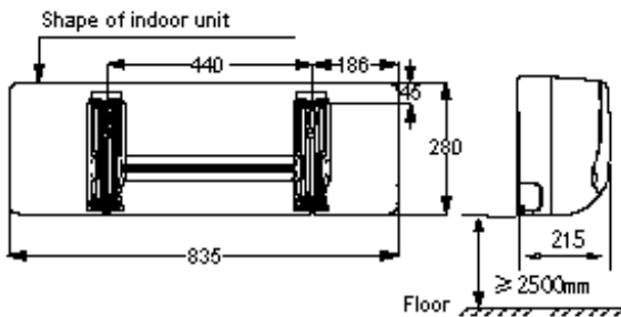
Figure 3.1: Wall mounted space requirements (unit: mm)
